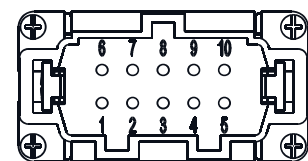
2 zones 10 PIN 16A230V Male & Female insert CNM10/CNF10
